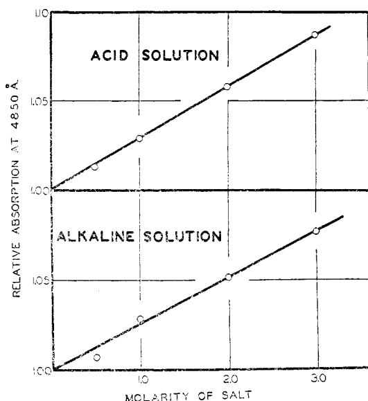
FIG. 3. Effect of salts (sodium chloride, sodium bromide, sodium chlorate, sodium nitrate, potassium chloride, potassium bromide) on light absorption of end forms of methyl orange (20).
