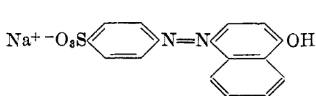
IX Orange I
