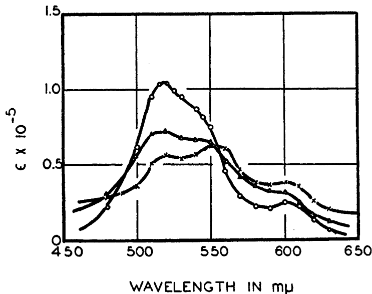
FIG. 6. Absorption spectra of pinacyanol: O, in aqueous solution; X, in aqueous solution containing cetylpyridinium chloride; Δ, in aqueous solution containing gelatin (19).
