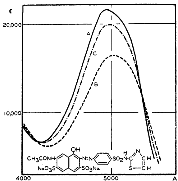
FIG. 17. Absorption spectra of azosulfathiazole: A, in buffer at pH 6.8; B, in buffer containing bovine albumin; C, in buffer containing bovine albumin and potassium acid phthalate.
