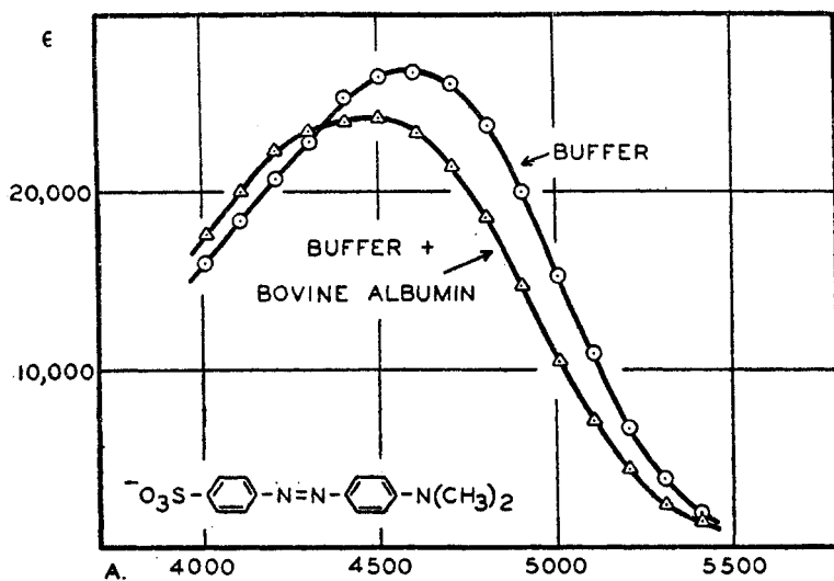
FIG. 15. Effect of serum albumin on spectrum of base form of methyl orange
