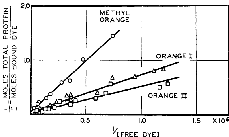
FIG. 14. Binding of some singly charged dyes by serum albumin at pH 5.7
