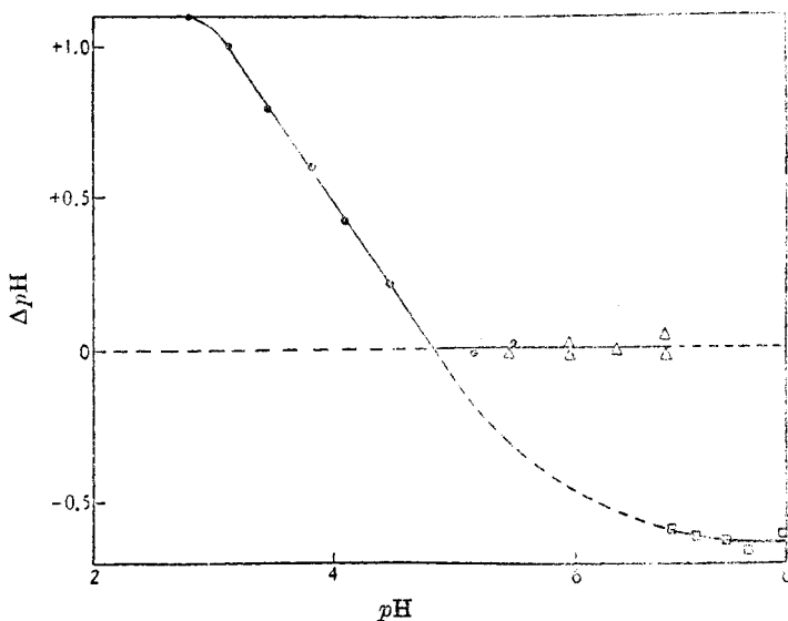
FIG. 10. Colorimetric pH errors in the presence of egg albumin: ●, bromocresol green; Δ, chlorophenol red; □, neutral red (2).
