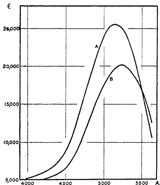
FIG. 18. Absorption spectra of amaranth: A, in buffer at pH 6.9; B, in buffer containing bovine albumin.
