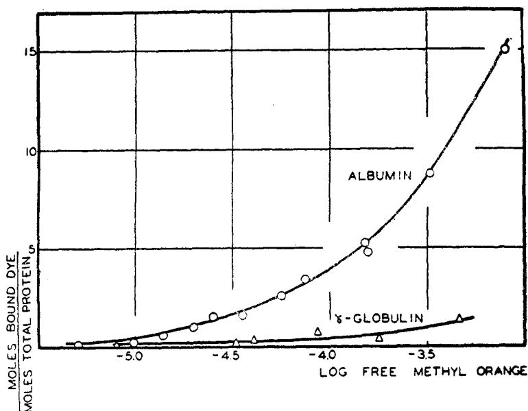
Fig. 12. Binding of methyl orange by serum proteins at pH 5.7
