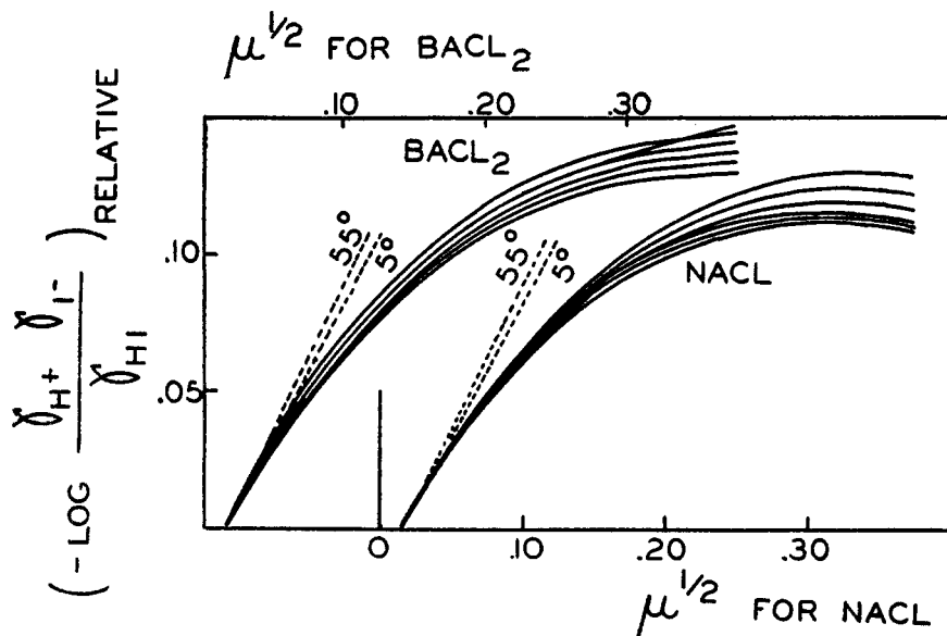
FIG. 4. Activity coefficient ratio (relative to reference solution) for methyl orange in solutions of sodium chloride and barium chloride, respectively. In each case the lowest curve is for 4.7°C., the others at higher temperatures, in intervals of 10°. The dotted lines represent the Debye-Hückel limiting slopes at the temperatures indicated (4, 21).
