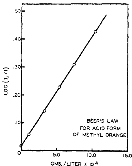
FIG. 7. Optical absorption of methyl orange 3 as a function of concentration, in acid solutions.
