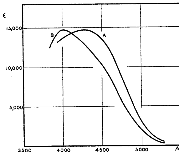
FIG. 20. Absorption spectra of methyl red: A, in buffer at pH 7.3; B, in buffer containing bovine albumin.
