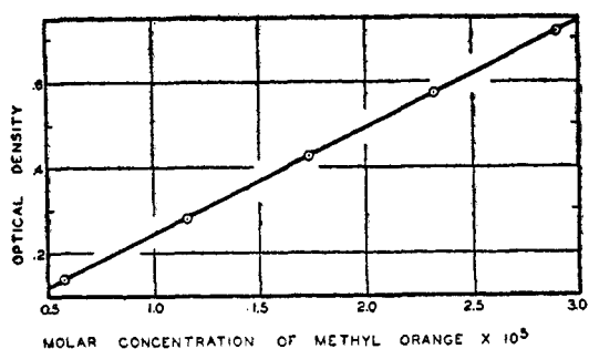
FIG. 8. 1 Optical absorption of methyl orange as a function of concentration in solutions of pH 5.7.
