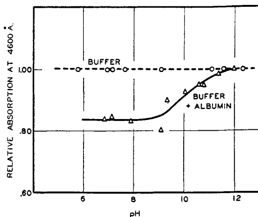
FIG. 21. Effect of pH on absorption spectra of methyl orange in albumin solutions
