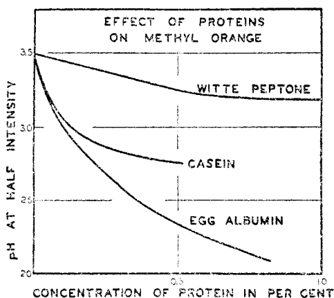
Fig. 9. Colorimetric pH errors of methyl orange in the presence of proteins (24)
