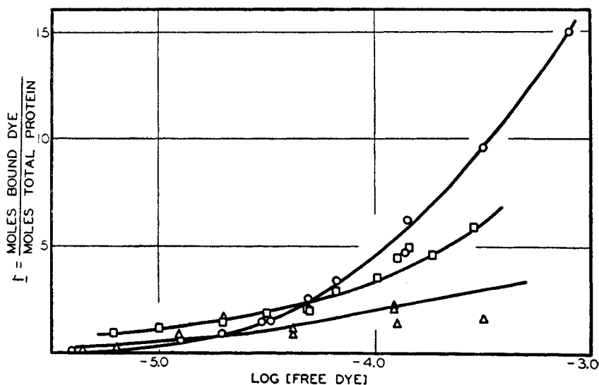
FIG. 13. Binding of sulfonate compounds by bovine serum albumin at pH 5.7; O, methyl orange (II); □, azosulfathiazole (XI); △, amaranth (XII).
