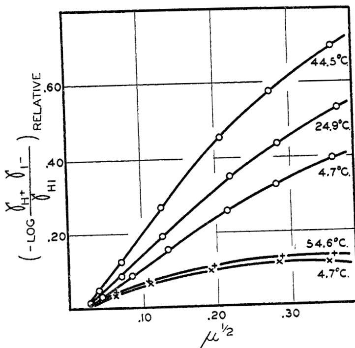
FIG. 5. Salt effect of sodium sulfate on absorption of methyl orange as a function of temperature: O, sodium sulfate; +, ×, sodium chloride.
