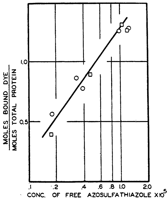
FIG. 19. Quantitative data on the extent of binding of azosulfathiazole: O, from spectral measurements; □, from dialysis-equilibrium studies.
