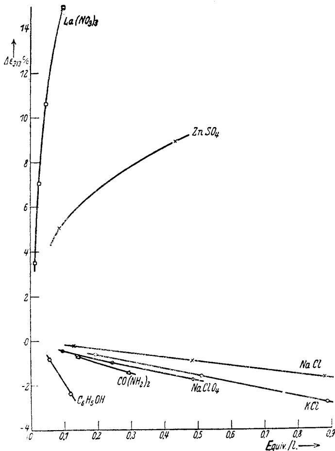
FIG. 2. Effect of various substances on the optical absorption of the 2,4-dinitrophenolate ion.
