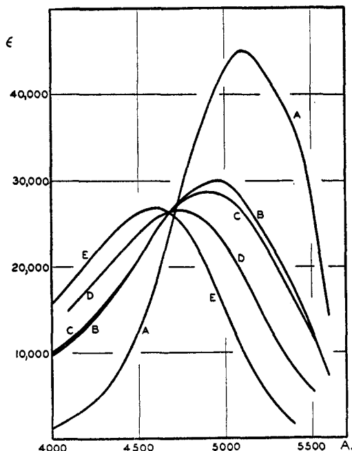
Fig. 1. Salt effects on spectra of methyl orange. A, indicator in solution of hydrochloric acid, pH 1.98; B, indicator in solution of hydrochloric acid, pH 3.51; C, indicator in solution B with addition of potassium chloride to give 0.25 molar solution; D, indicator in solution B with addition of sodium sulfate to give 0.06 molar solution; E, indicator in phosphate buffer, pH 7.73.
