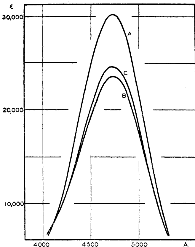
FIG. 16. Absorption spectra of Orange I: A, in buffer at pH 6.8; B, in buffer containing bovine albumin; C, in buffer containing bovine albumin and potassium acid phthalate.
